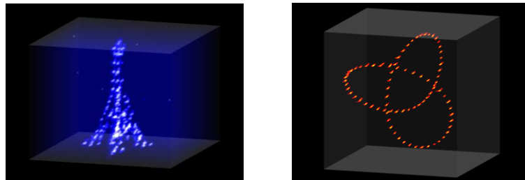
Fluorescence images of individual atoms trapped in various optical tweezers arrays. Each point corresponds to an atom.
